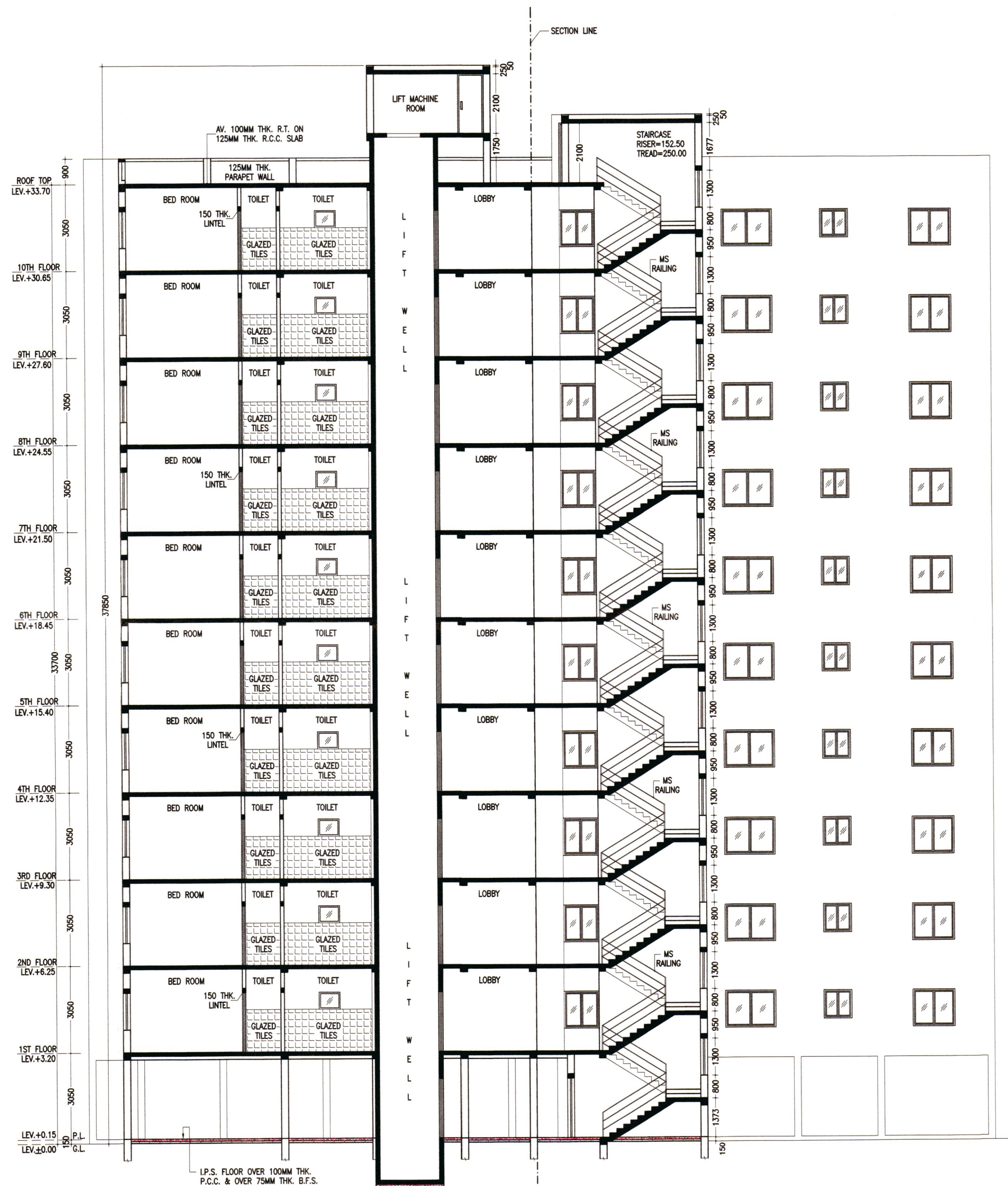
SECTION-A-A SCALE-1:100
